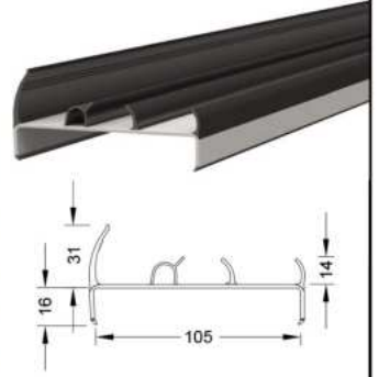
FRİGOFİRİK KAPI FİTİLİ Refrigerated vehicle door seal
