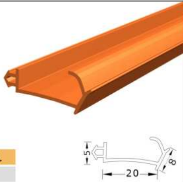
KASA/KANAT CONTASI Frame and wing seal
