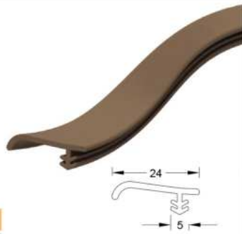
KASA/KANAT CONTASI Frame and wing seal
