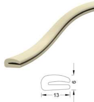
PANO KAPAK KENAR FİTİLİ Board Cover Edge Seal
