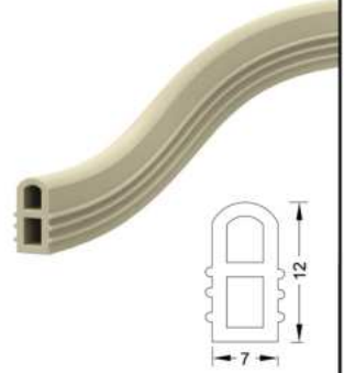
YEMEK DOLABI KAPAK LASTİĞİ Rubber Cover For Food Cabinet
