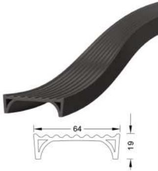
DEPO SIRT LASTİĞİ Back Of The Fuel Tank Fixings
