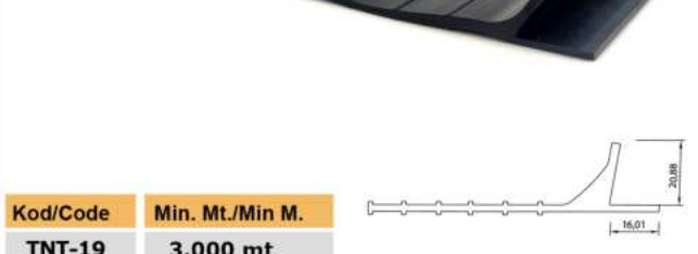
KEPENK PANJUR FİTİLİ Shutter seal
